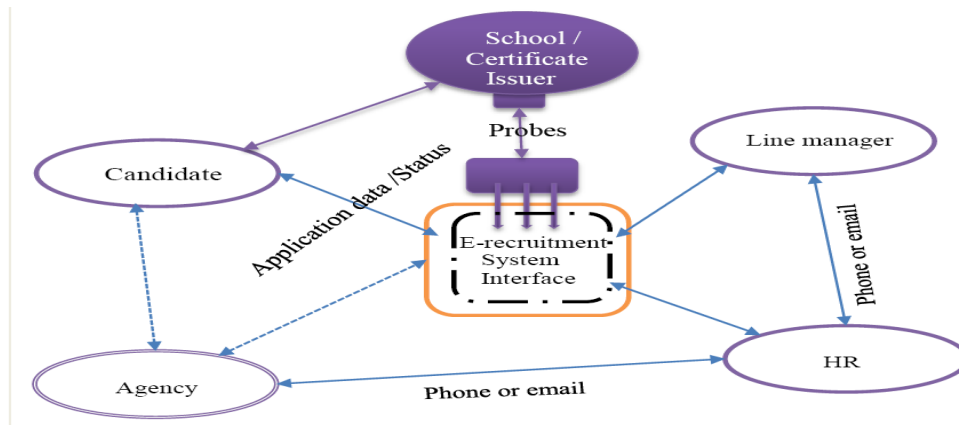
Figure 1: E-Verification .....
